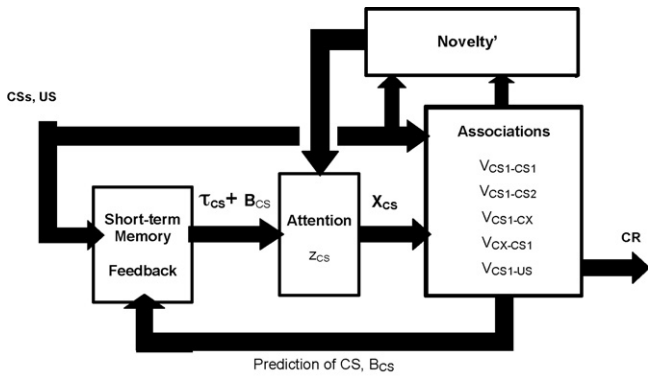
Fig. 1. Block diagram of the Schmajuk–Lam–Gray (SLG [13]) network. CS: conditioned stimulus; US: unconditioned stimulus; \tau_{CS} : short-term memory trace of the CS; B_{CS} : prediction of the CS; z_{CS} : attentional memory; X_{CS} : internal representation of the CS; V_{CS1-CS1} , V_{CS1-CS2} , ..., V_{CS1-US} : associations CS1–CS1, CS1–CS2, ..., CS1–US; CR: conditioned response.
