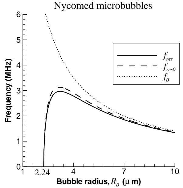
FIG. 2. Resonance frequency (solid) of an air microbubble encapsulated by a polymeric shell 25,27 as a function of the outer radius of the microbubble, compared with the undamped natural frequency (dotted). The microbubble resides in human blood plasma. The dashed line is the resonance frequency under the assumption that blood plasma is incompressible [Eq. (29)]. The solid and dotted lines are calculated from Eqs. (30) and (18), respectively. The encapsulating shell is characterized by viscosity of 0.45 \text{ Pa}\cdot\text{s} and elasticity of 12 \text{ MPa} . Its thickness is 5% of the bubble outer radius. Other parameters: \mu_l = 0.0012 \text{ Pa}\cdot\text{s} , C_l = 1543 \text{ m}\cdot\text{s}^{-1} , \rho_{l0} = 1027 \text{ kg}\cdot\text{m}^{-3} , \rho_{s0} = 1100 \text{ kg}\cdot\text{m}^{-3} , p_0 = 0.1 \text{ MPa} , \sigma_1 = 0.04 \text{ N}\cdot\text{m}^{-1} , \sigma_2 = 0.005 \text{ N}\cdot\text{m}^{-1} , and \kappa = 1.1 .
