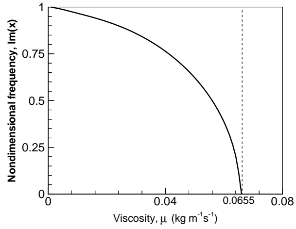
FIG. 2. Quadropule shape oscillations of a purely viscous liquid drop: frequency versus shear viscosity. Parameters: R = 0.1 mm, \rho_l = 10^3 \text{ kg m}^{-3} , \sigma = 0.073 \text{ kg s}^{-2} , \text{De}_1 = \text{De}_2 = 0 .
