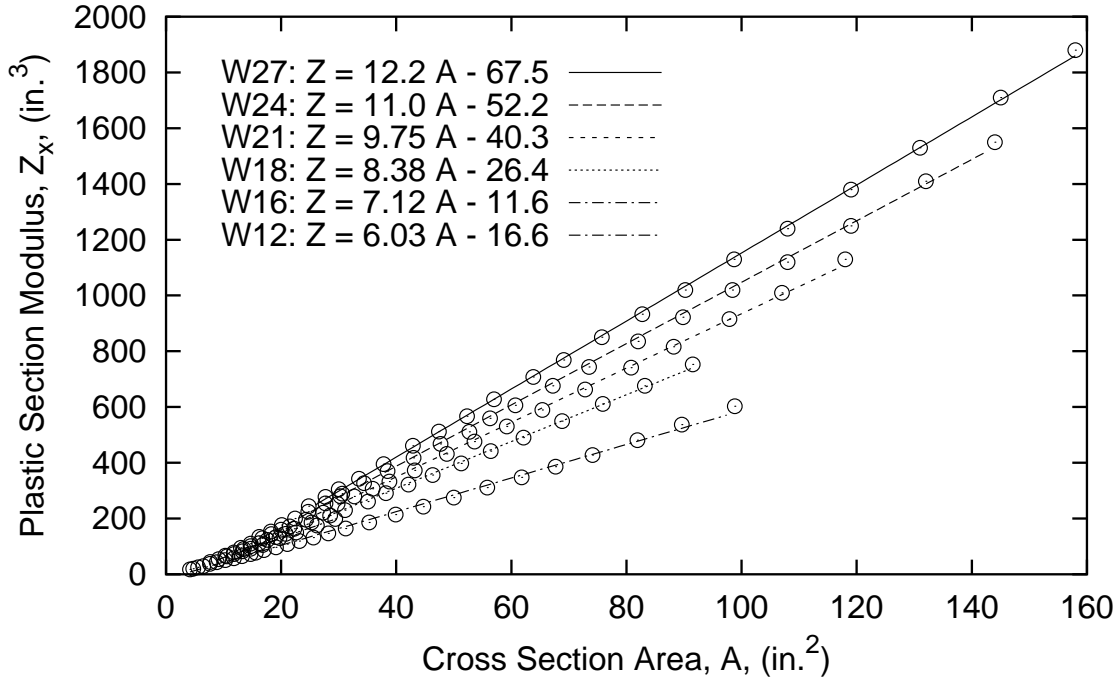
relationship between cross section area and plastic section modulus
